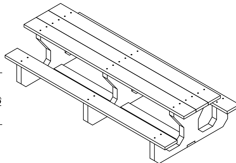
3D ISOMETRIC VIEW
